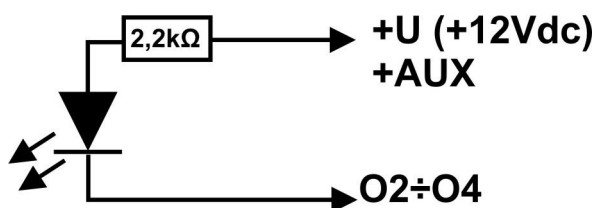
Dioda LED
